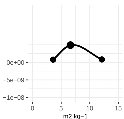
psnTOpt
