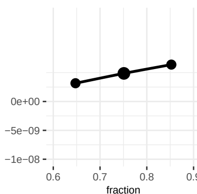
half_saturation_PAR
