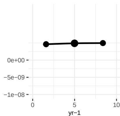
leafC
