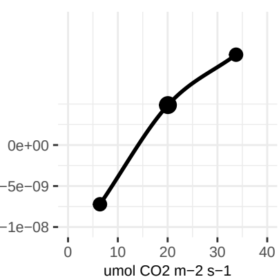
Vm_low_temp
