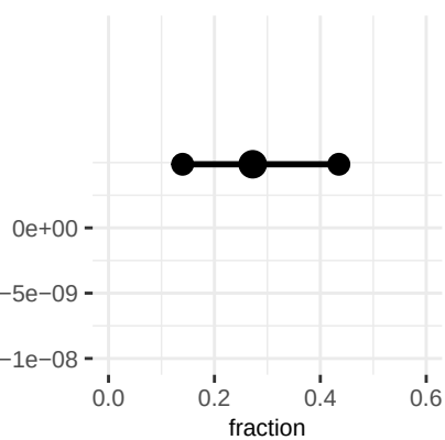
Amax
