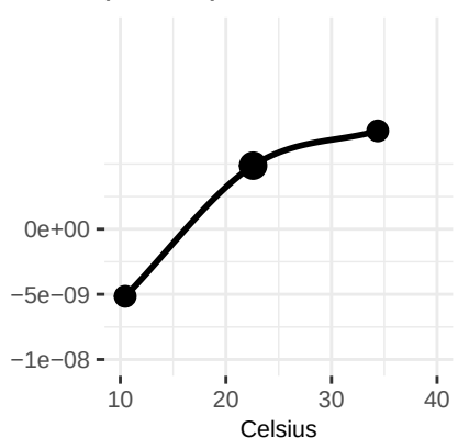
dVPDSlope
