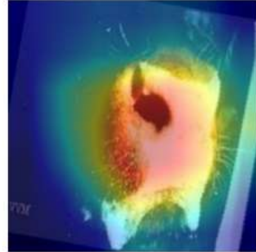
MobileNetV2 Grad-CAM
