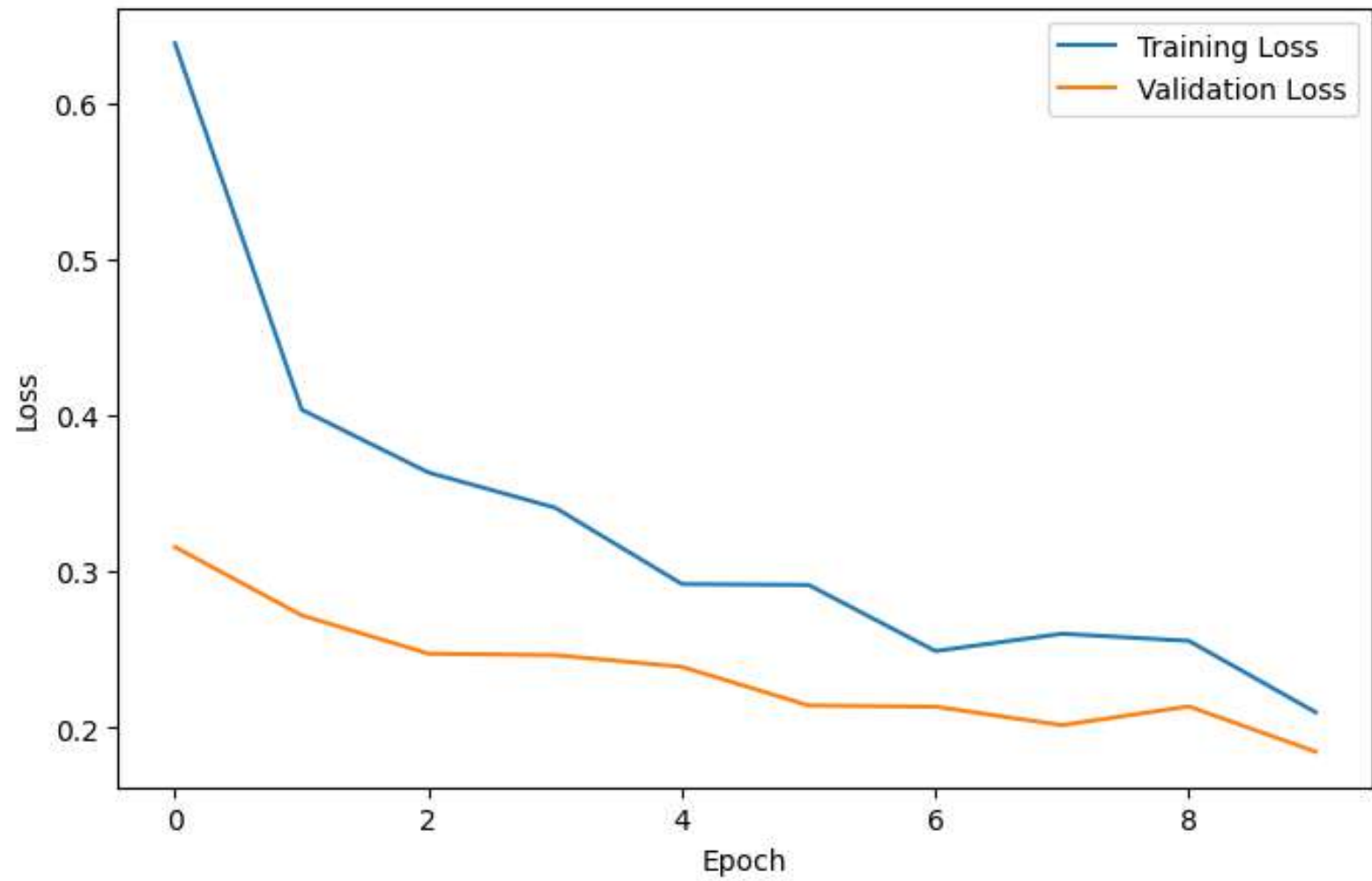
MobileNetV2 Loss
