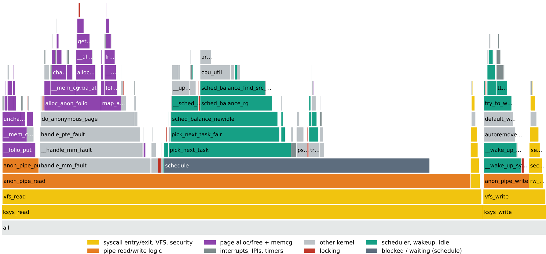
fttrace function_graph: kernel time under read() and write(), 4 KB messages
