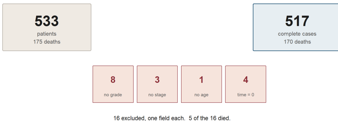
Figure 2: From 533 patients to the 517-patient nested cohort. The 16 exclusions are drawn separately: 8 lack grade, 3 lack stage, 1 lacks age, and 4 have survival time zero. 5 of those 16 died. Stage-only and grade-only sensitivities restore the grade-missing and stage-missing patients (525 and 520).
