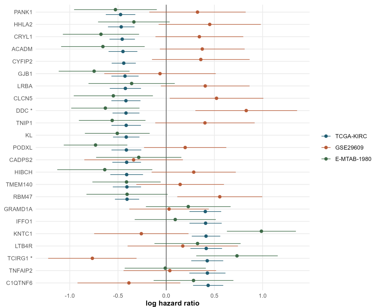
Figure 5: Log hazard ratios for the high-confidence genes in TCGA-KIRC, GSE29609 (17 deaths), and E-MTAB-1980 (23 deaths). DDC and TCIRG1 are marked. Direction agreement is not the same as a confidence interval that excludes zero.
