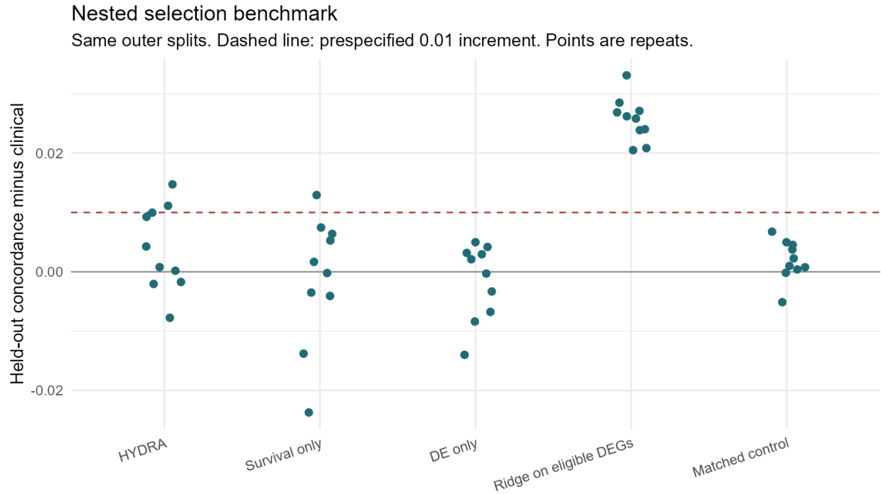
Figure 3: Held-out concordance minus the clinical model for five selectors on the same outer repeats. The dashed line is the prespecified 0.01 threshold. Points are repeats; intervals are reported in the text.
