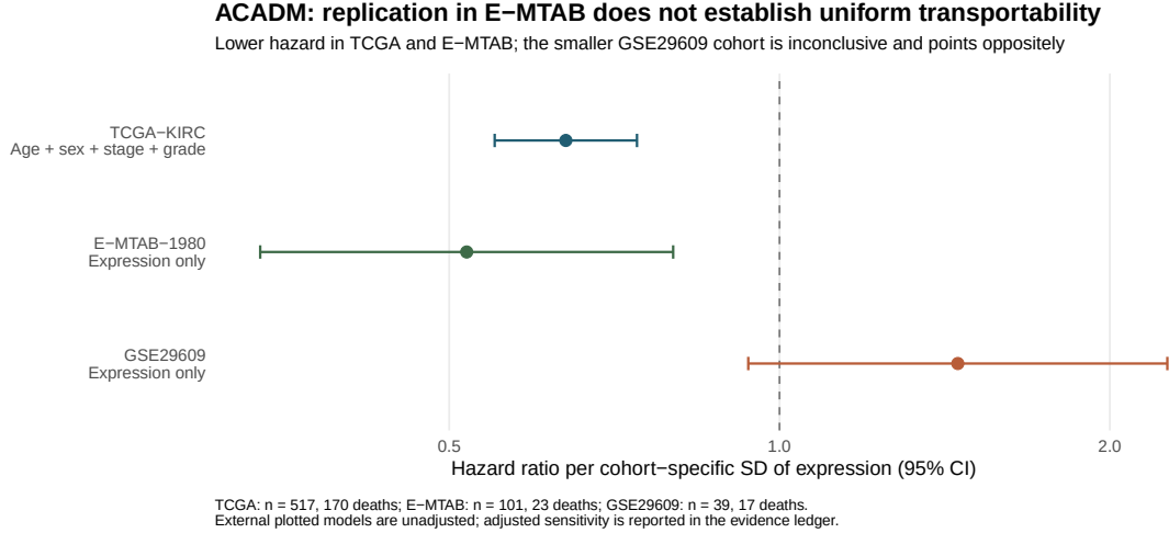
Figure 2: Representative cohort-specific agreement for ACADM. Hazard ratios and 95% intervals use continuous expression. TCGA adjusts for age, sex, stage, and grade; external estimates are unadjusted. Standardization uses cohort-specific expression scales, so effect magnitudes are not a common assay-scale contrast. E-MTAB-1980 supports the TCGA direction, while GSE29609 does not. Both external cohorts were previously inspected.
