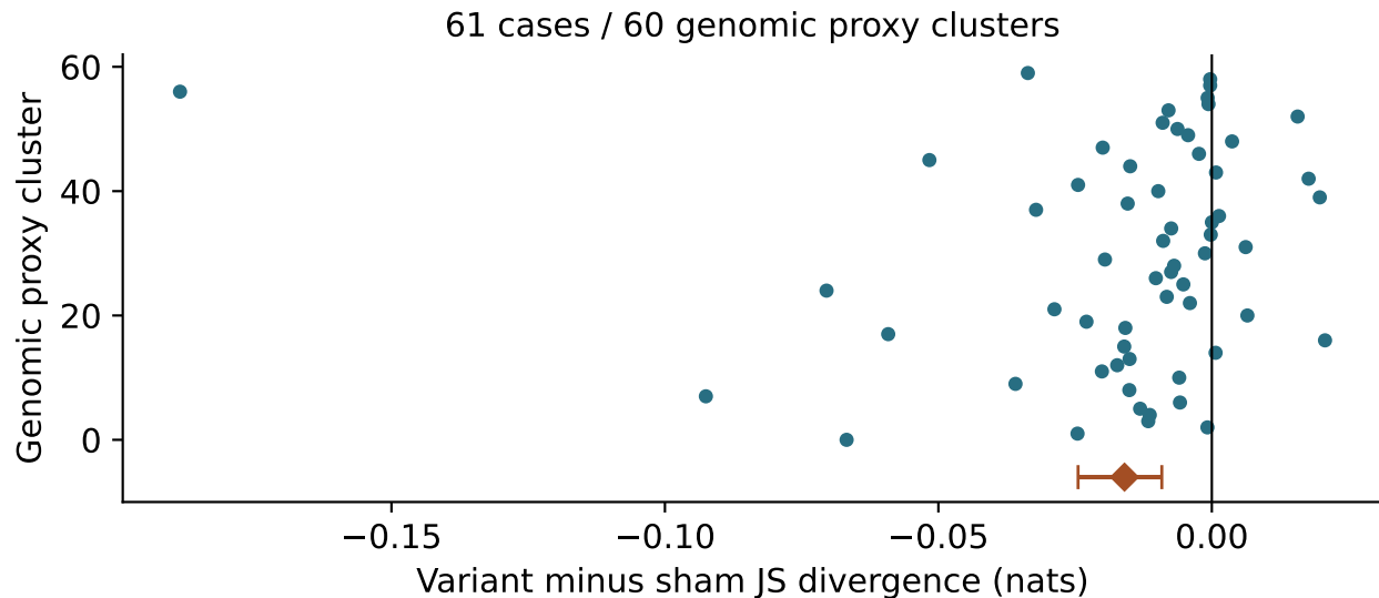
Figure 1: Variant-minus-sham contrasts in Jensen–Shannon divergence for 61 cases in 60 genomic proxy clusters. Blue points show cluster means in saved table order; vertical position is a display index, not a biological measurement. The diamond and bar show the equal-cluster mean and 95% cluster-bootstrap interval in nats, conditional on the fixed checkpoint and eligibility rules.
