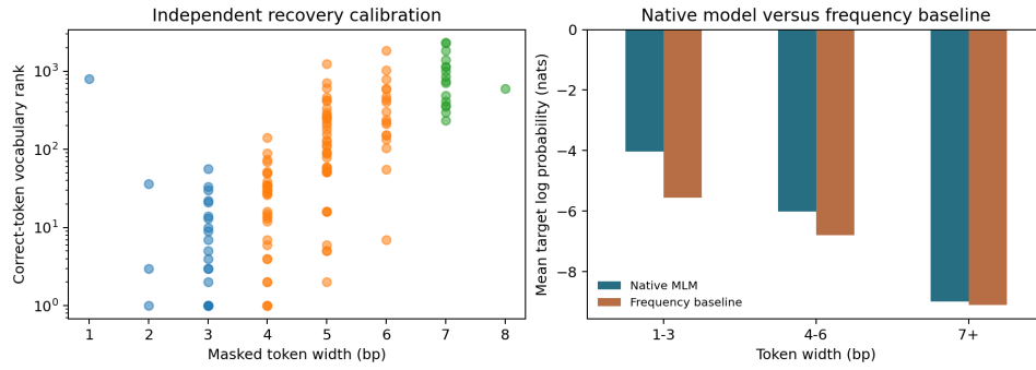
Figure 6: Independent masked-token recovery on 128 fixed chromosome 16/17 windows. Vocabulary rank and log probability depend on token width; comparison uses a smoothed token-frequency baseline from chromosomes 14/15. This calibrates recovery competence without testing motif-specific sensitivity.
