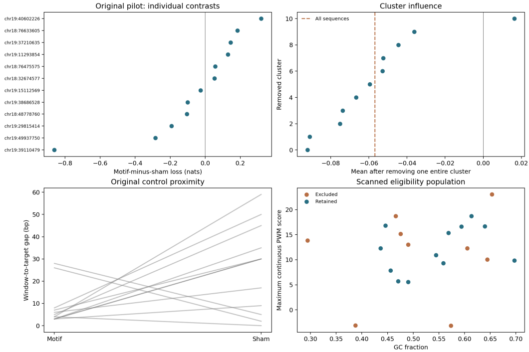
Figure 5: Discovery-pilot geometry, eligibility and cluster influence. Leave-cluster-out estimates remove every sequence in the omitted genomic cluster; changing signs indicate sensitivity to membership.
