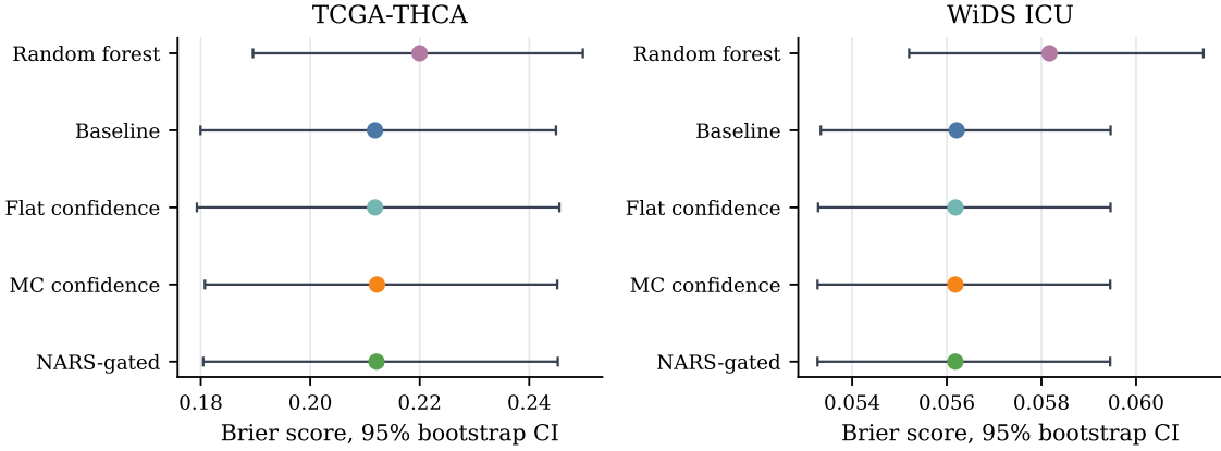
Figure 2: Held-out Brier scores with 95% bootstrap confidence intervals. Lower values are better. The transformer variants are close, so small point-estimate differences should be interpreted together with paired-bootstrap comparisons.
