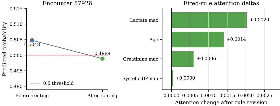
Figure 4: Generated case-trace visualization for selected WiDS held-out encounter 57926. The left panel shows the near-threshold probability before and after routing; the right panel shows attention changes for 4 fired rules.
