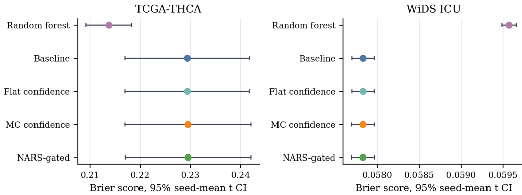
Figure 2: Current five-seed mean Brier scores with 95% Student- t intervals over training seeds on fixed held-out cases. These are seed-mean intervals, not case-bootstrap intervals or external confirmation.
