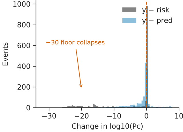
Fig. 1. Frozen test histograms of later movement y - \text{risk} and unguarded XGBoost residual y - \hat{y} . The spike at 0 is reports that do not move. The left tail is collapse to the dataset floor -30 .
