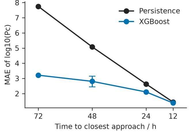
Fig. 2. Forecast-horizon MAE for unguarded XGBoost and persistence. Whiskers at 48 h are the 95% bootstrap interval on the MAE gap, shown on the XGBoost point.
