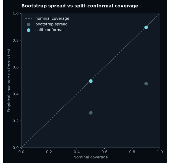
Fig. 2. Nominal versus empirical coverage for bootstrap spread and split conformal (frozen test).
