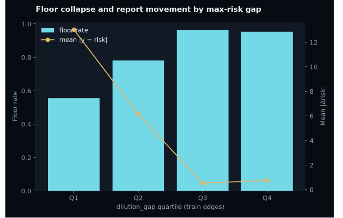
Fig. 4. Floor rate and mean |y - \text{risk}| by train-quartile of the max-risk gap (frozen test).
