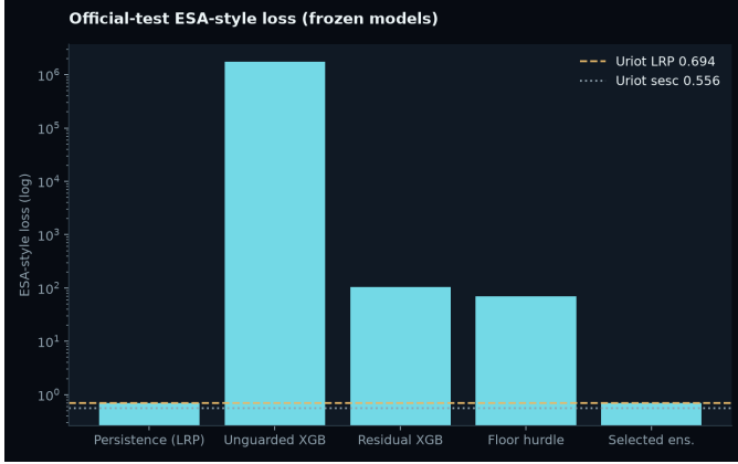
Fig. 3. Official-test ESA-style loss for frozen models versus Uriot last-risk-prediction (0.694) and sesc (0.556). Log scale.
