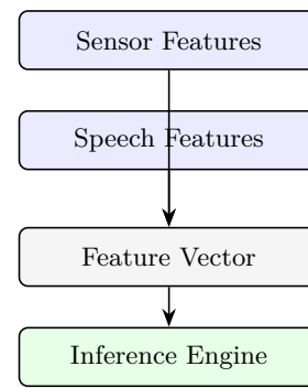
Figure 19: Data fusion: timestamp-aligned sensor and speech features are combined into a single feature vector for the inference engine.
