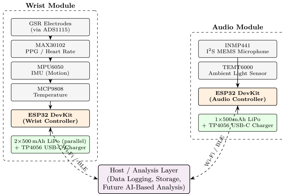
Figure 1: High-level system architecture of PSYCON, showing the Wrist Module (physiological sensing) and Audio Module (speech and environmental sensing) as independently powered ESP32-based subsystems that communicate wirelessly with a host/analysis layer.
