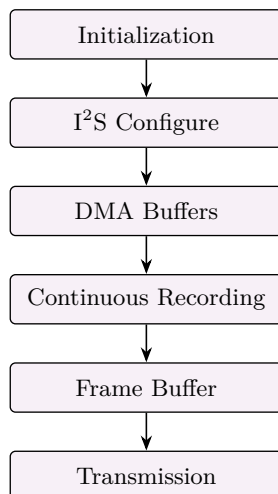
Figure 12: Audio Module acquisition pipeline: initialization, I²S configuration, DMA buffer setup, continuous recording, frame buffering, and transmission.
