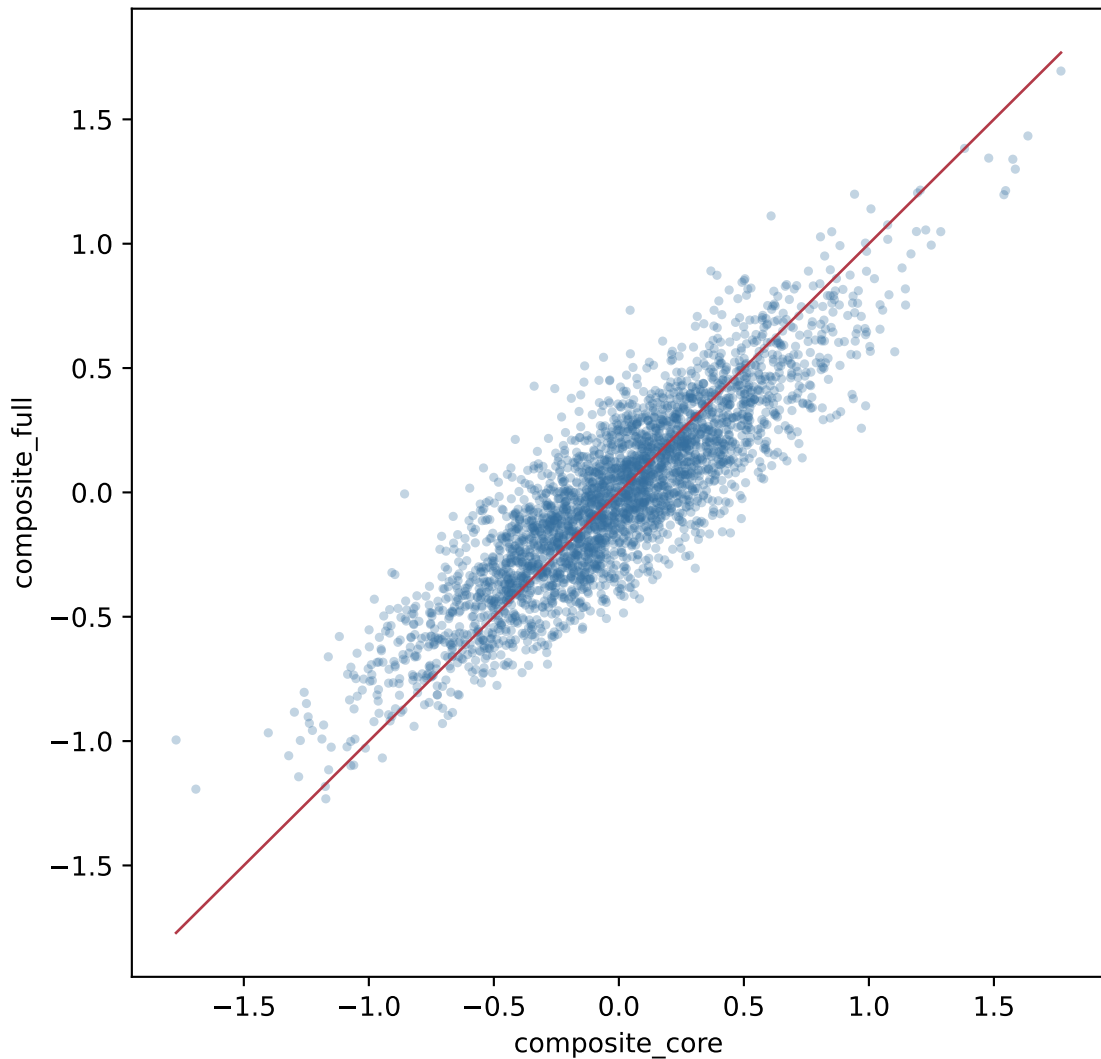
Core vs Full composite (Pearson r=0.869 , n=3164 )
