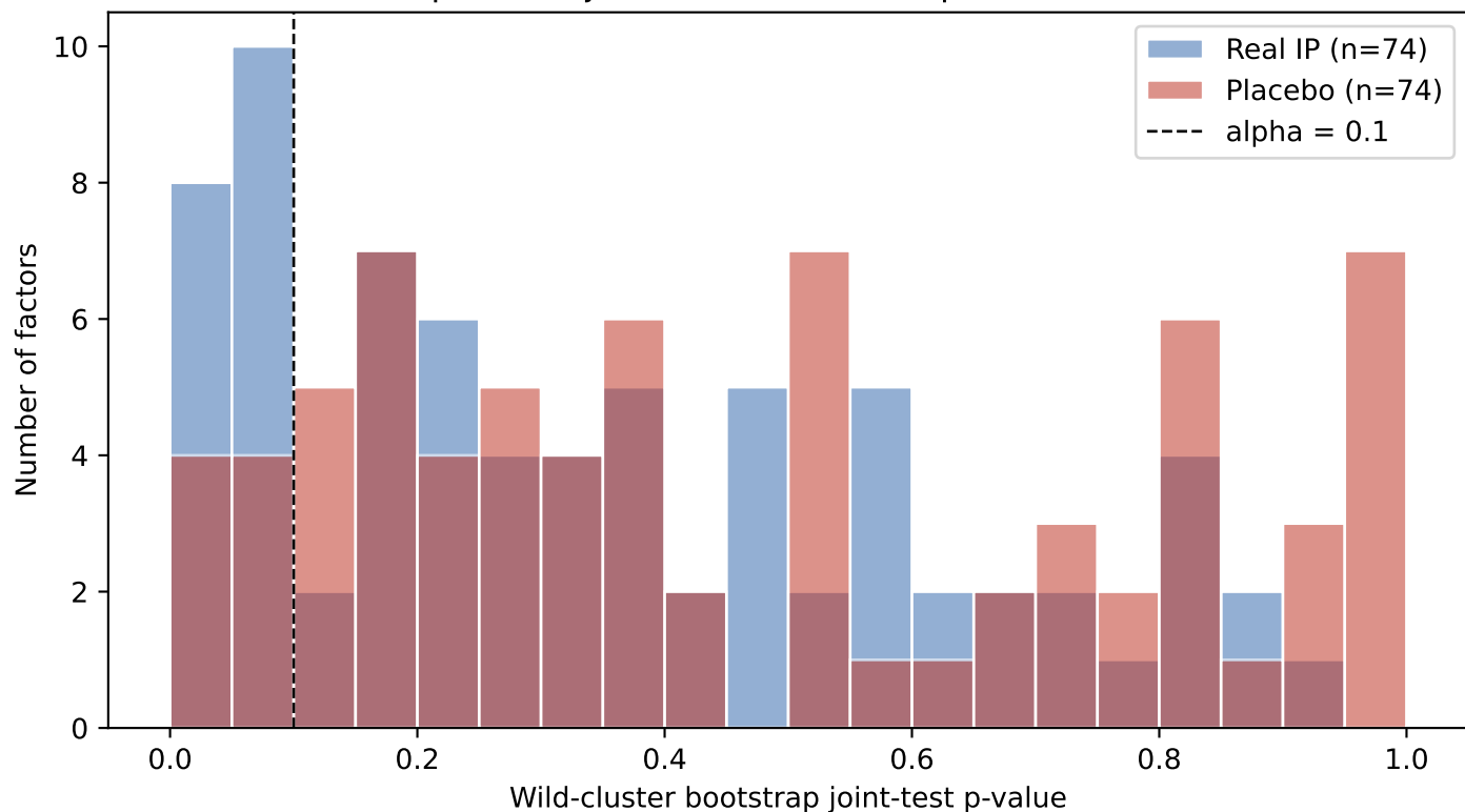
Real vs placebo: joint interaction-test p-values (IP branch)
