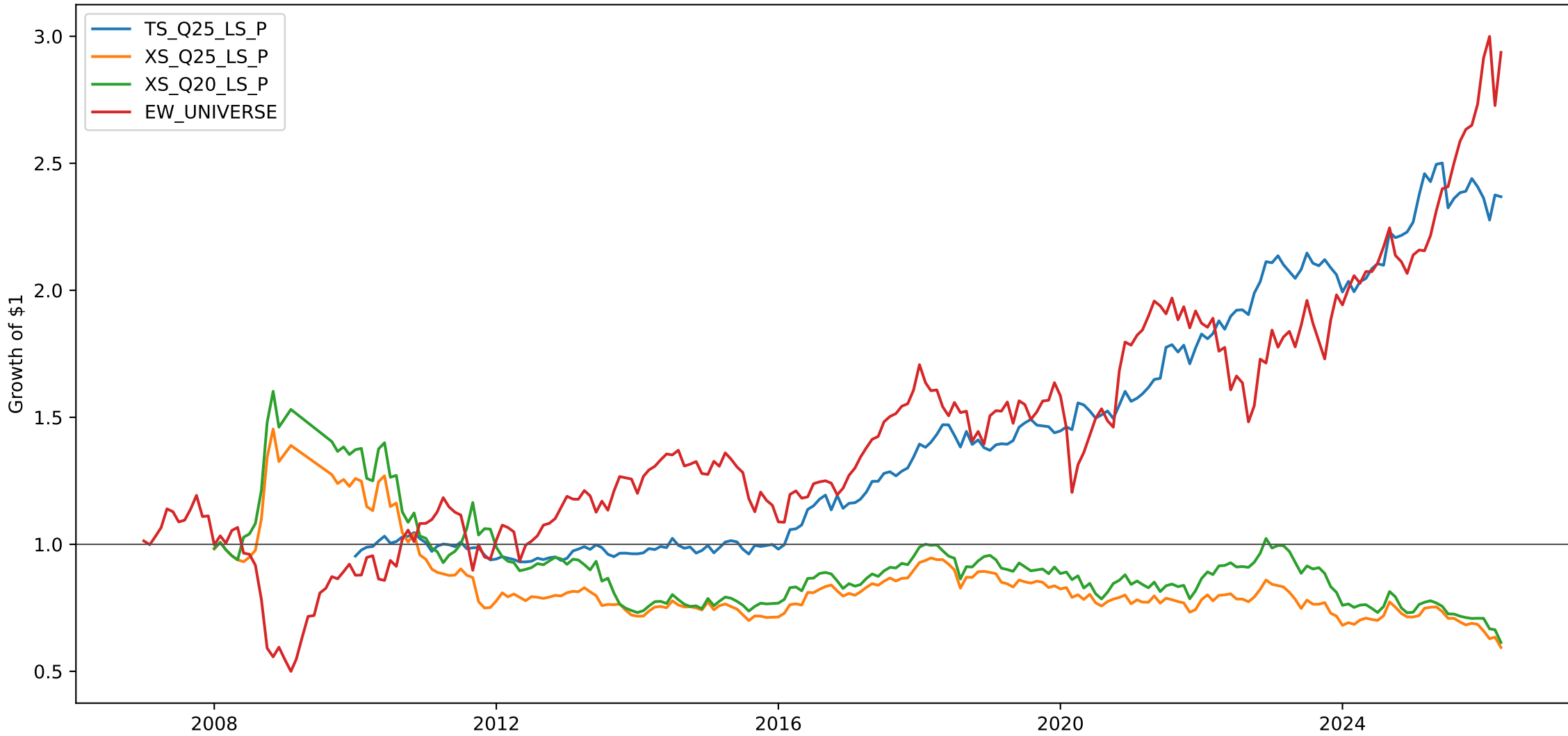
Contrarian P(adverse) strategy cumulative gross returns
