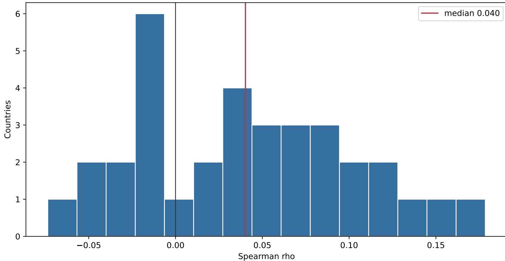
Per-country Spearman: P(adverse) vs 1M forward return
