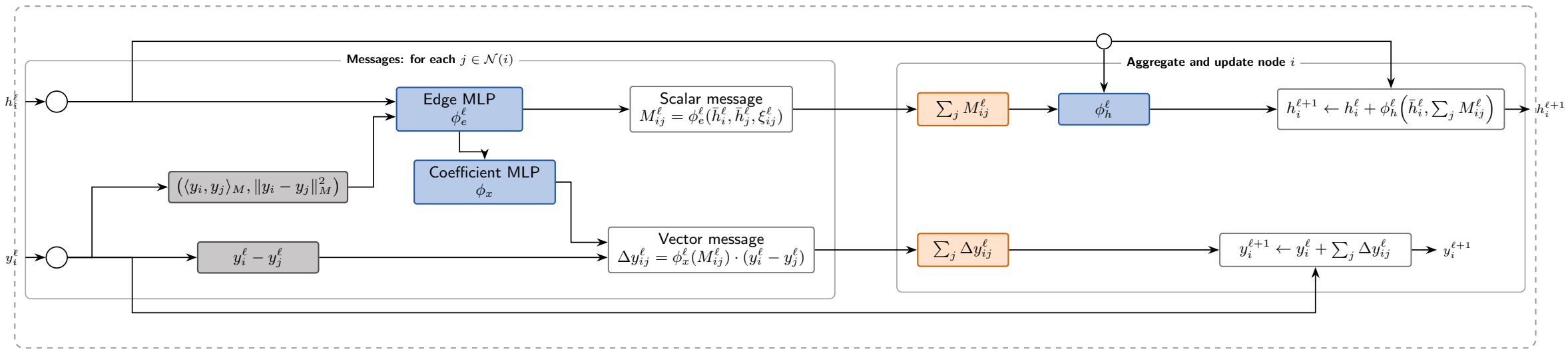
JetFUEL message-passing layer \ell
