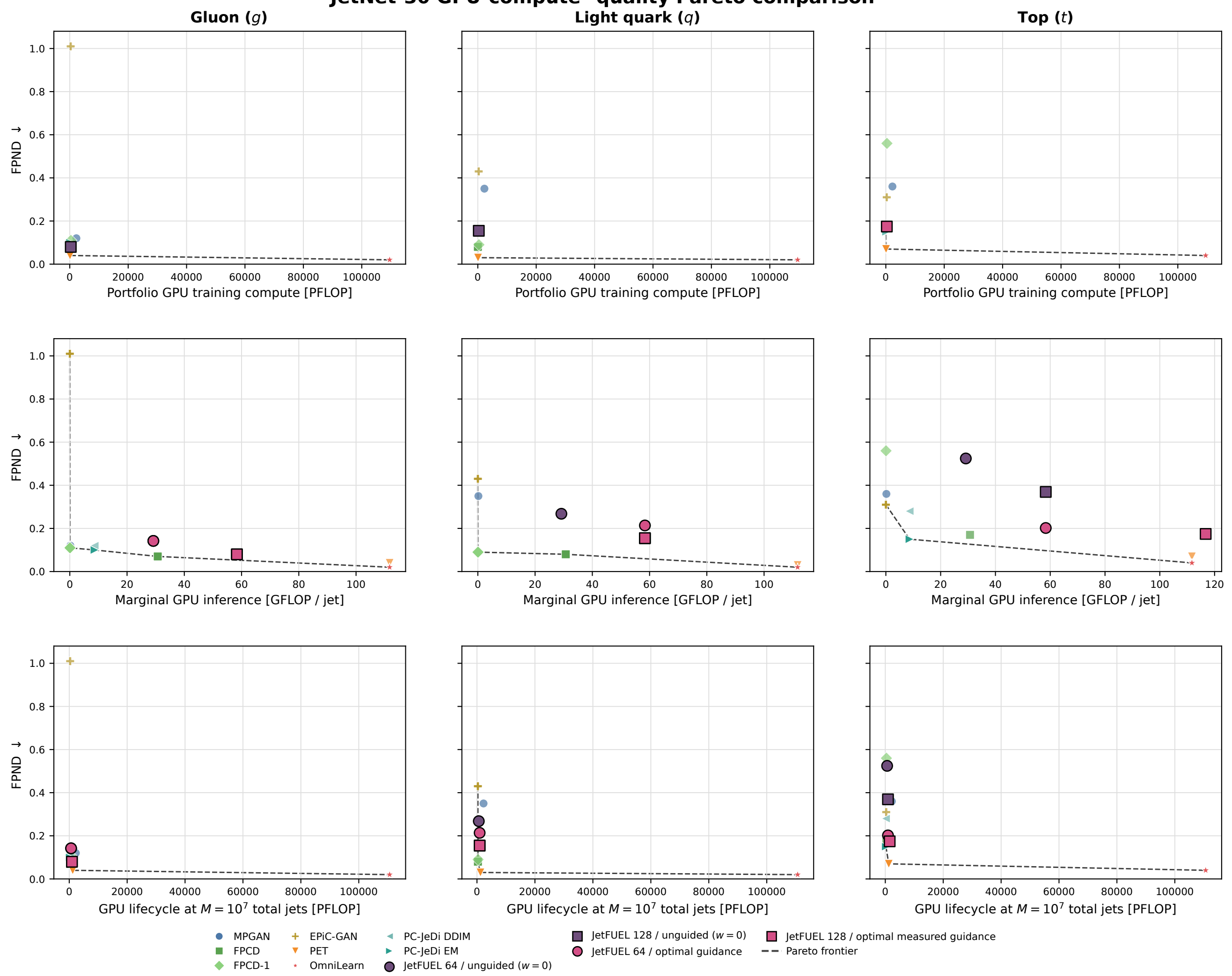
JetNet-30 GPU-compute--quality Pareto comparison
