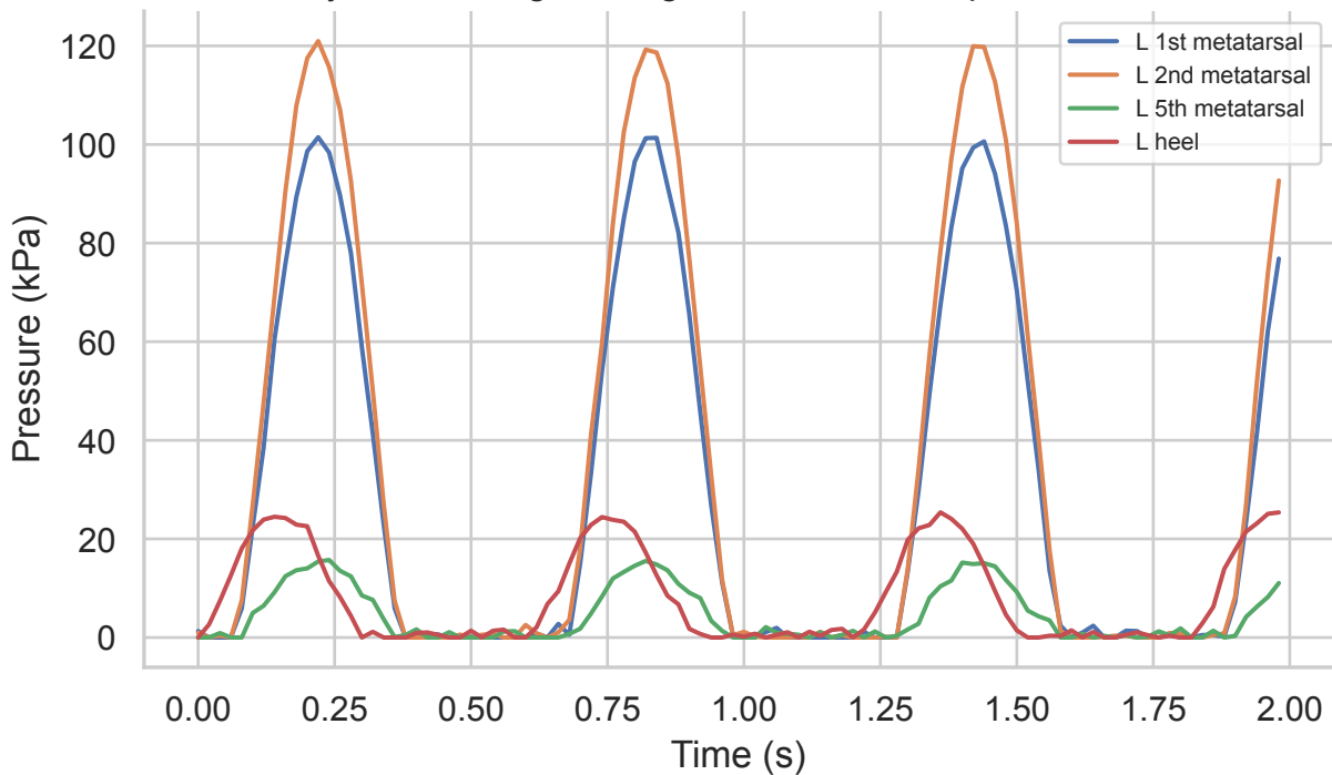
Simulated left-foot traces (one overload pattern) Synthetic / engineering validation — not patient data.
