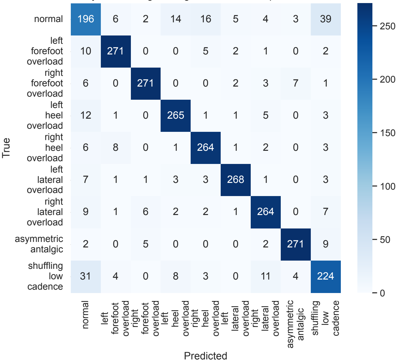
Grouped-CV confusion (logistic regression) Synthetic / engineering validation — not patient data.
