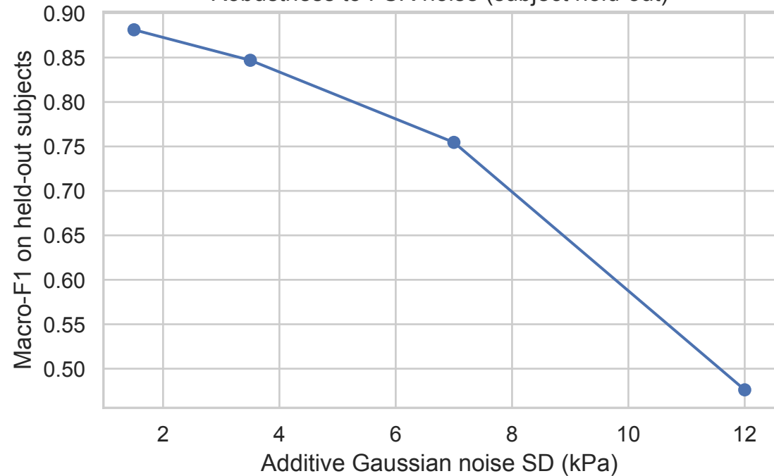
Robustness to FSR noise (subject hold-out)
