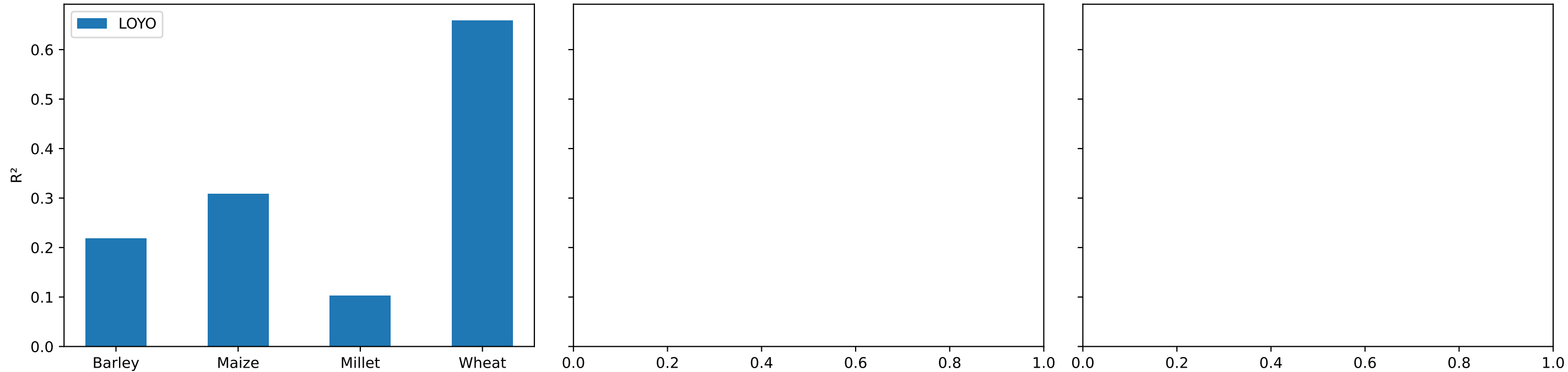
ANN (Combined)
