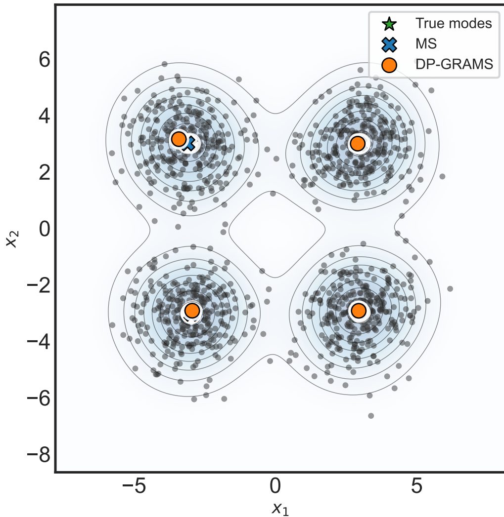
Mode Estimation for 4-Modal Bivariate Gaussian Mixture
