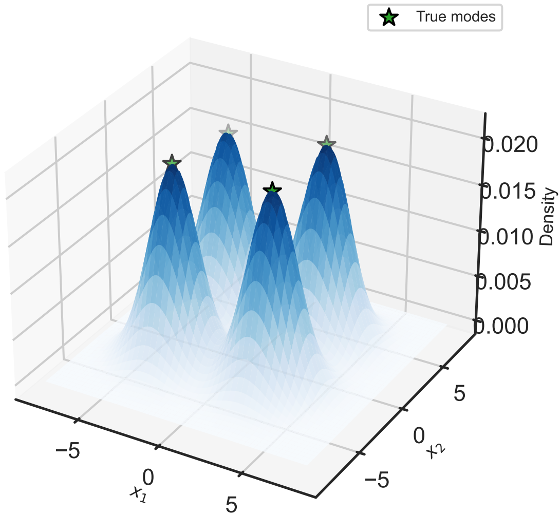
Estimated KDE Surface for 4-Modal Bivariate Gaussian Mixture
