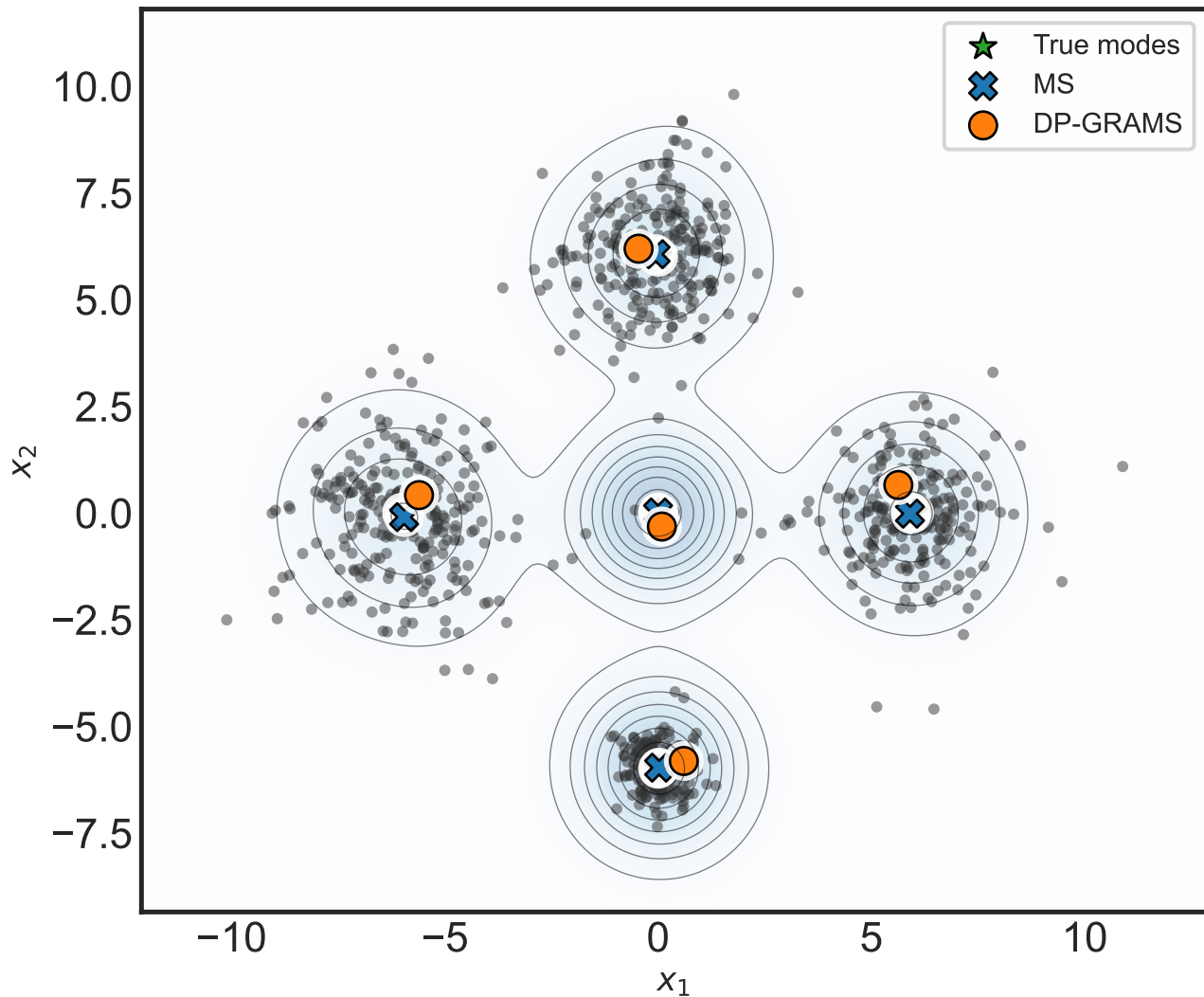
Mode Estimation for 5-Modal Bivariate t-Mixture
