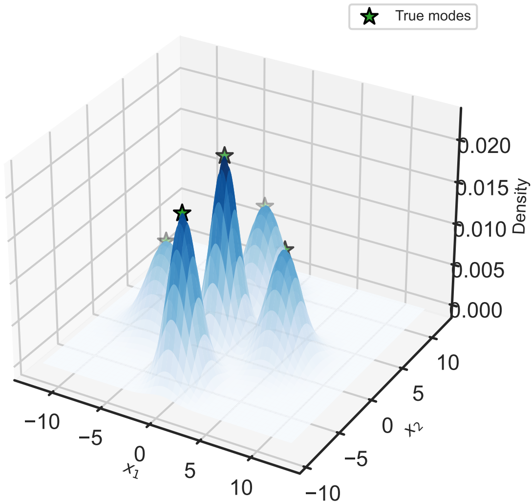
Estimated KDE Surface for 5-Modal Bivariate t-Mixture
