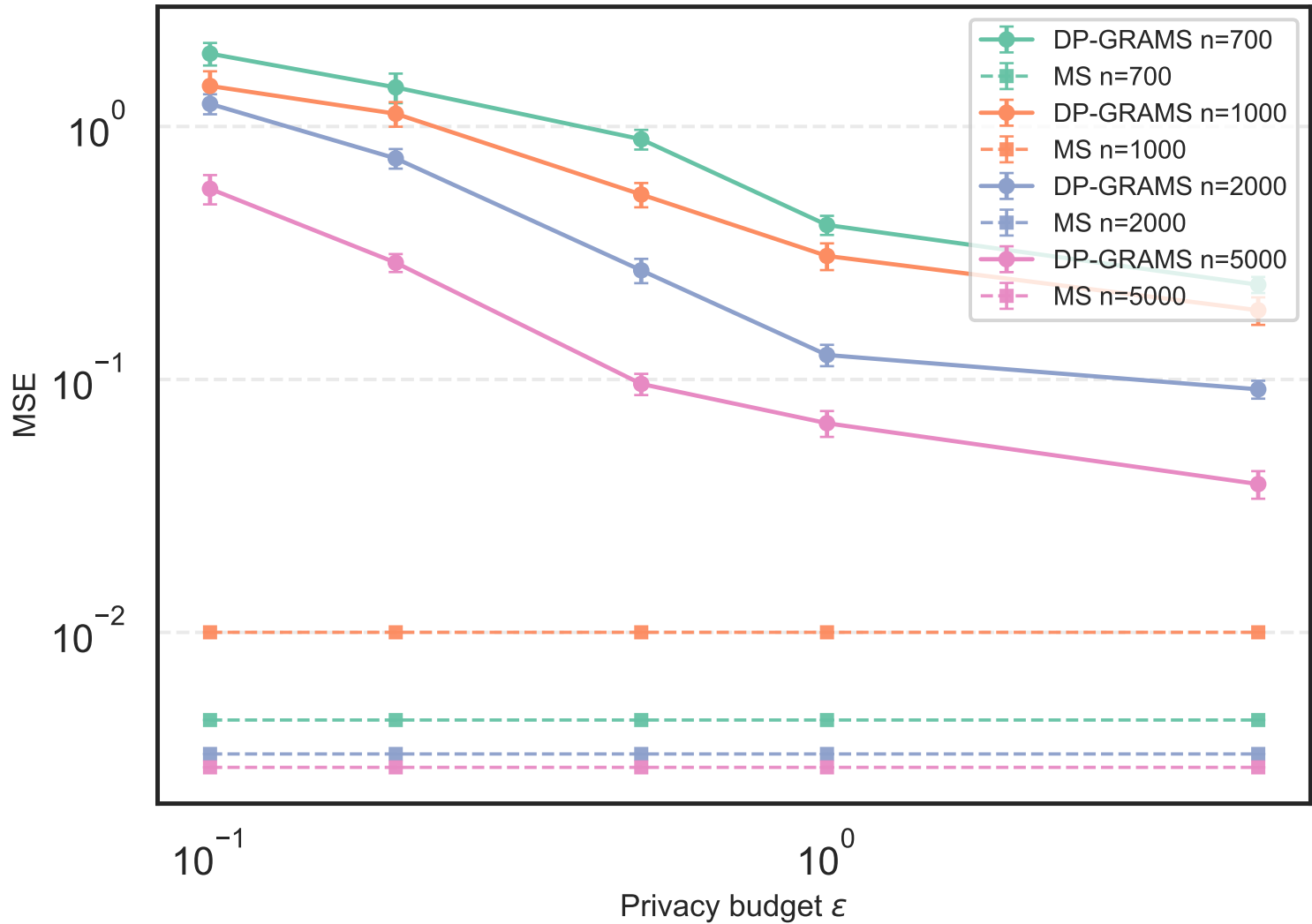
Privacy-Utility Tradeoff for 5-Modal Bivariate t-Mixture
