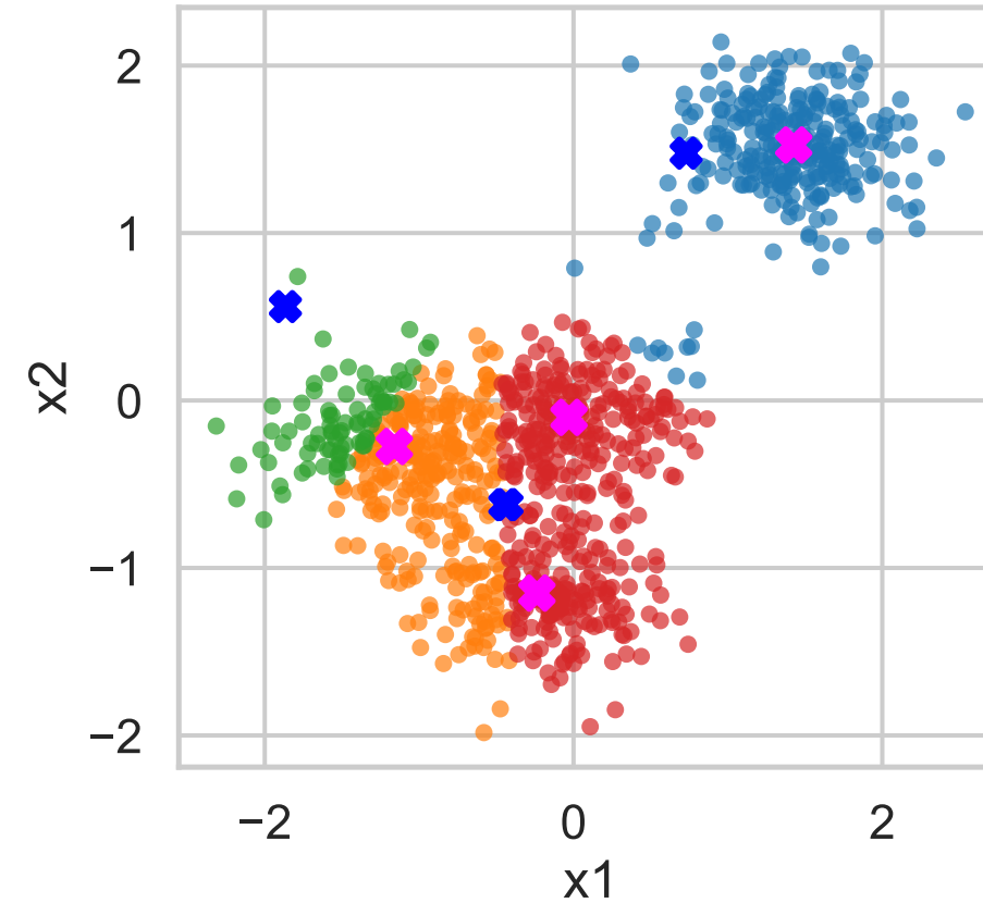
DP-KMeans
