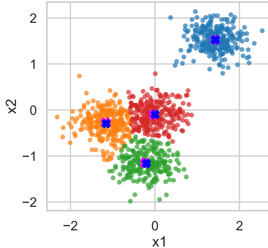
KMeans
