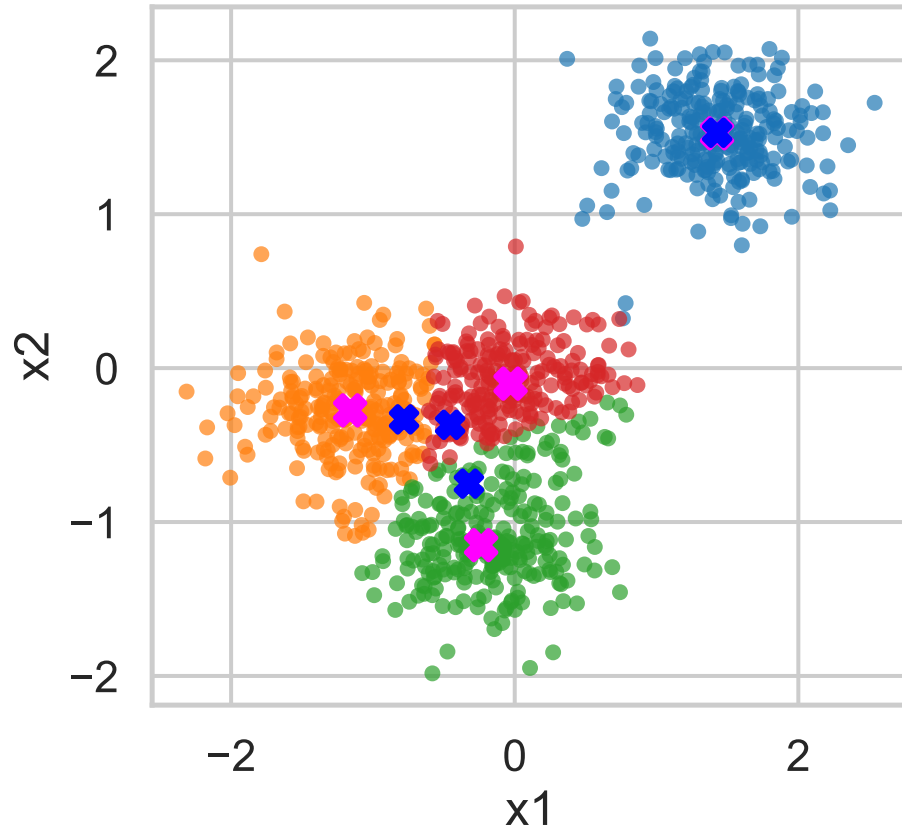
MS Clustering
