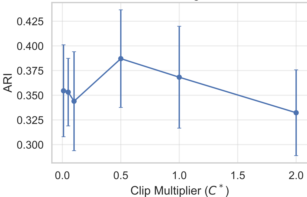
DP-GRAMS-C on Digits: ARI vs C^*
