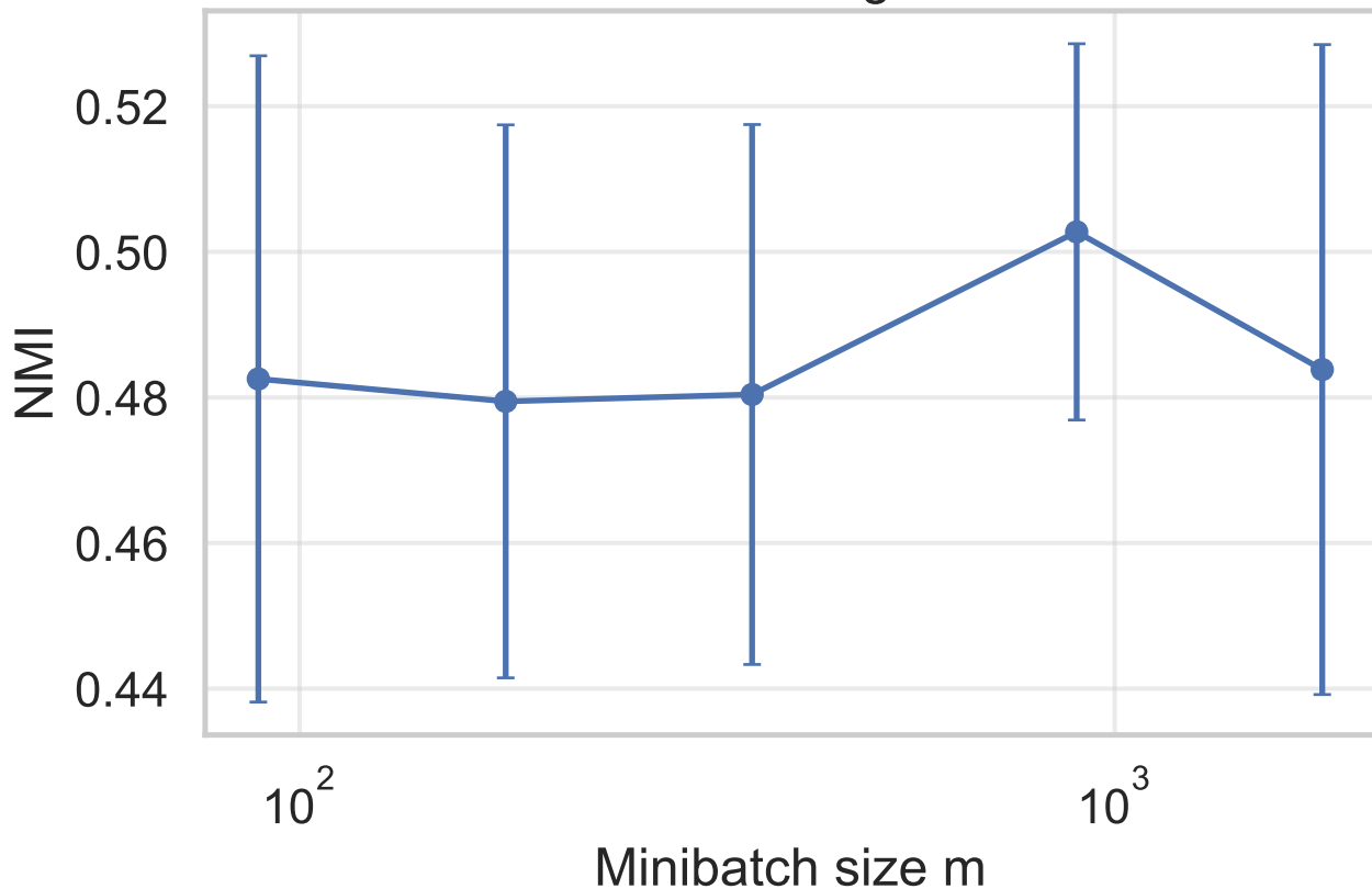
DP-GRAMS-C on Digits: NMI vs m
