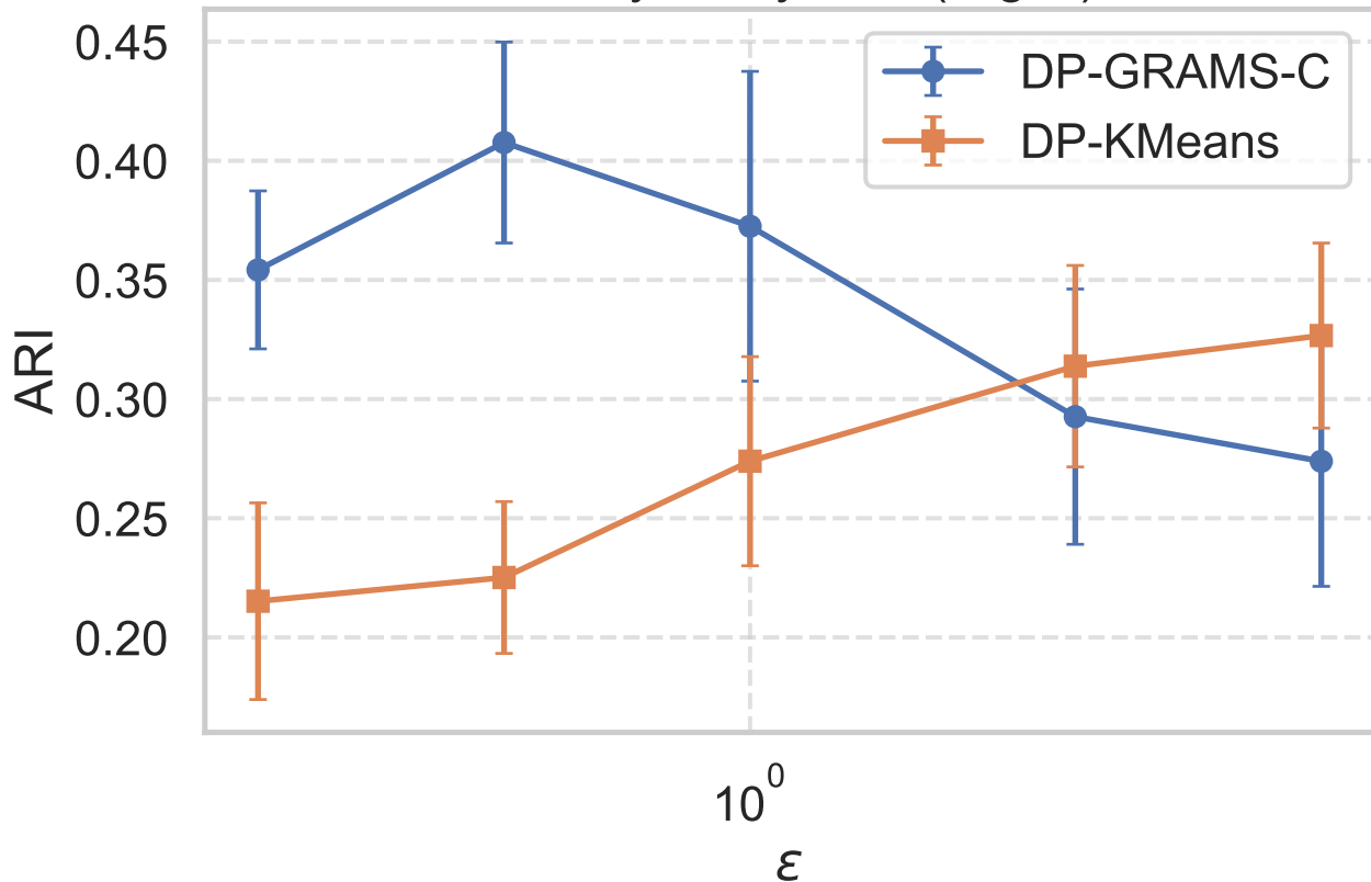
Privacy-Utility: ARI (Digits)
