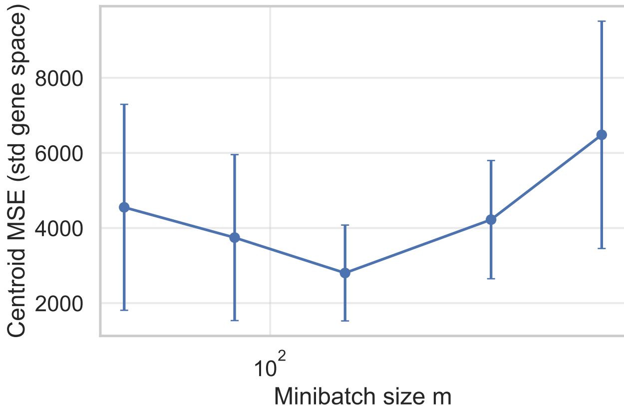
DP-GRAMS-C on Gene: Centroid vs m
