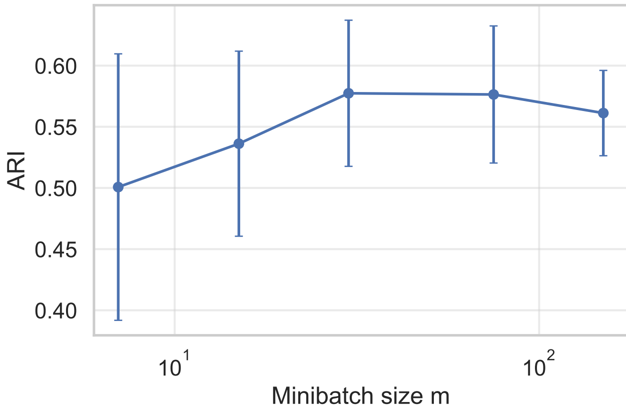
DP-GRAMS-C on Iris: ARI vs m
