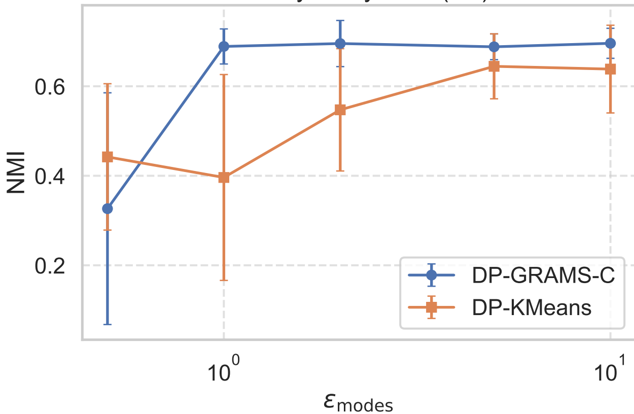
Privacy-Utility: NMI (Iris)
