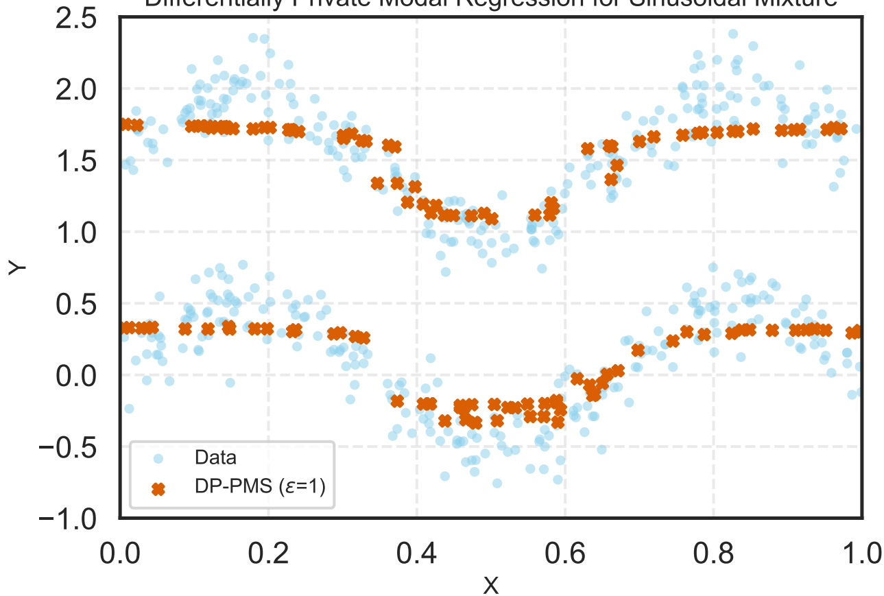
Differentially Private Modal Regression for Sinusoidal Mixture
