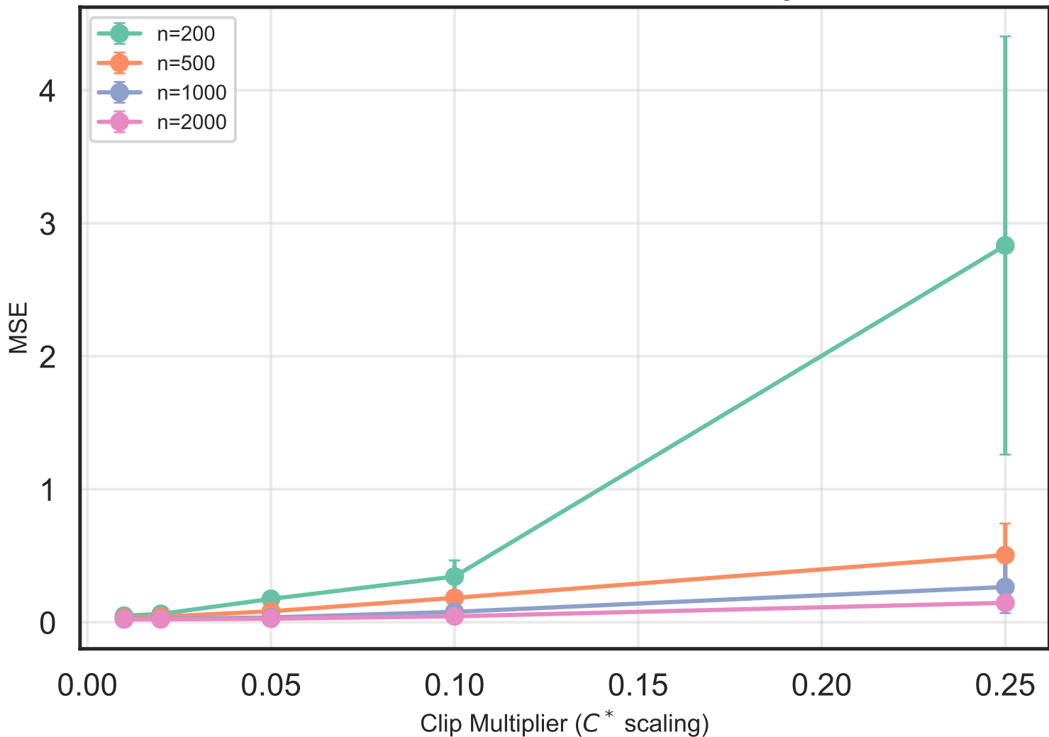
MSE vs C^* across n for Sinusoidal Modal Regression
