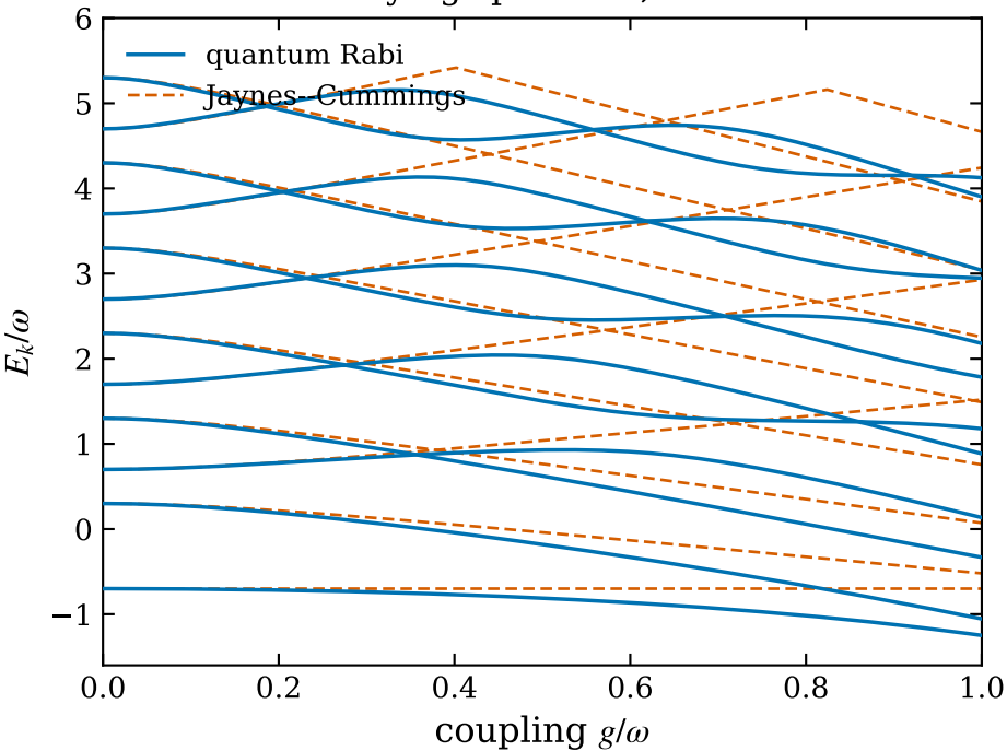
Low-lying spectrum, \Delta = 0.7 \omega
