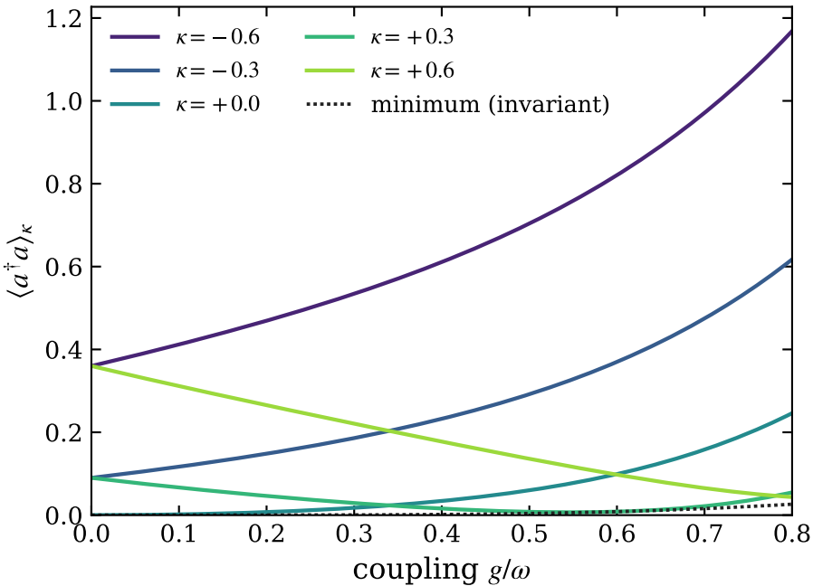
Photon number across gauges, \Delta = 0.7 \omega
