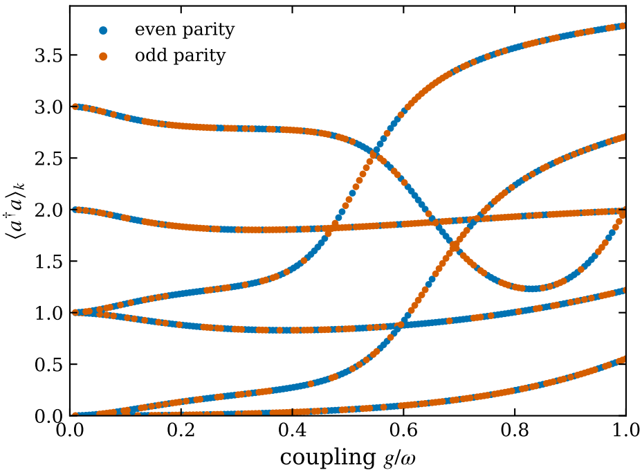
Photon content of the lowest eigenstates, \Delta=0.7\omega
