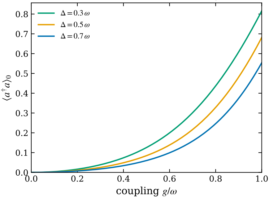
Ground-state photon number (exact diagonalisation)
