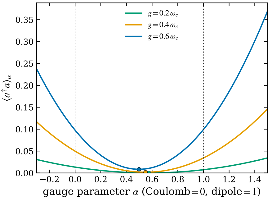
Unit-curvature gauge orbit (dots: invariant minima)
