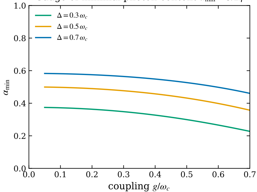
Gauge of minimal photon content \alpha_{\min} = C/2\eta
