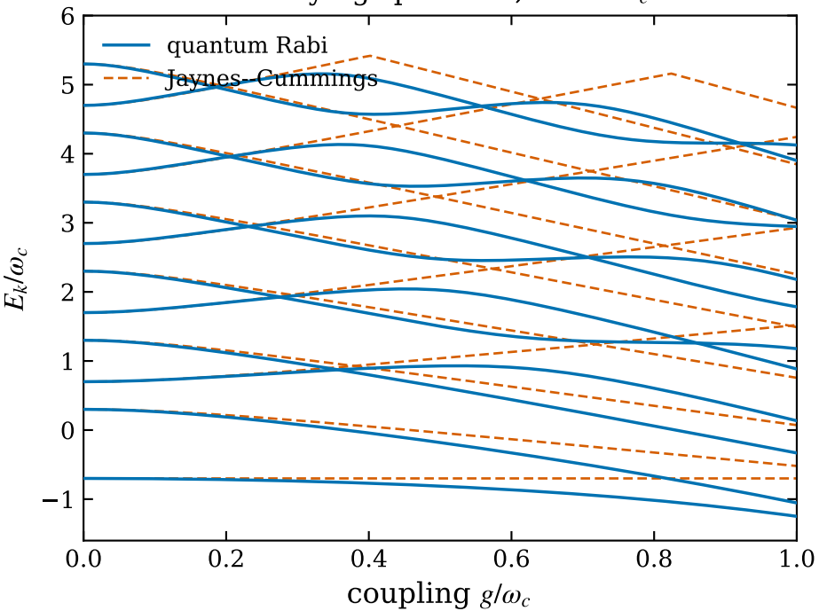
Low-lying spectrum, \Delta = 0.7 \omega_c
