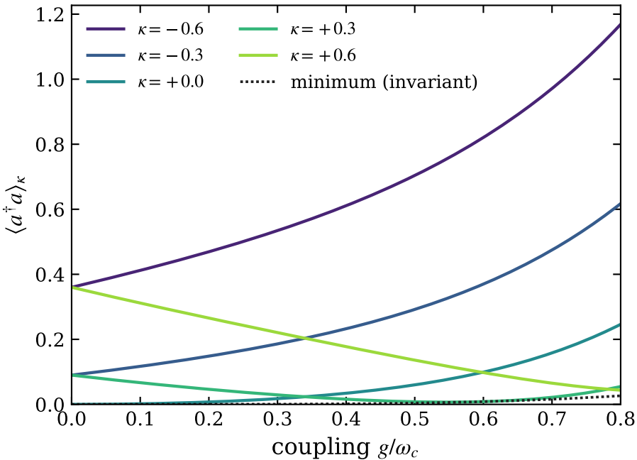
Photon number across gauges, \Delta = 0.7 \omega_c
