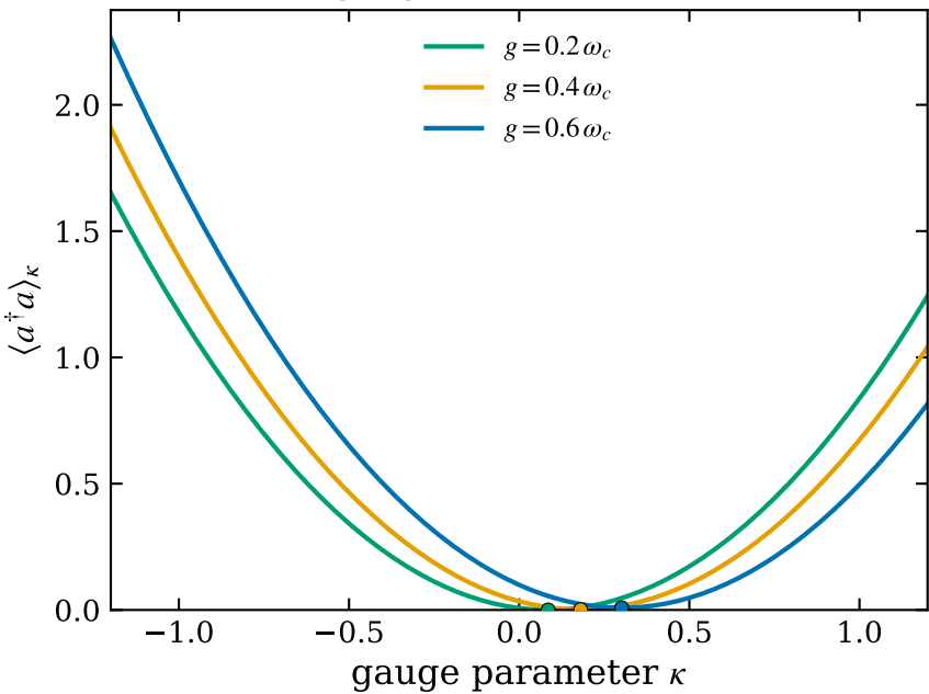
Unit-curvature gauge orbit (dots: invariant minima)
