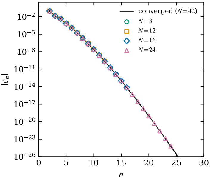
Convergence of the coefficients
