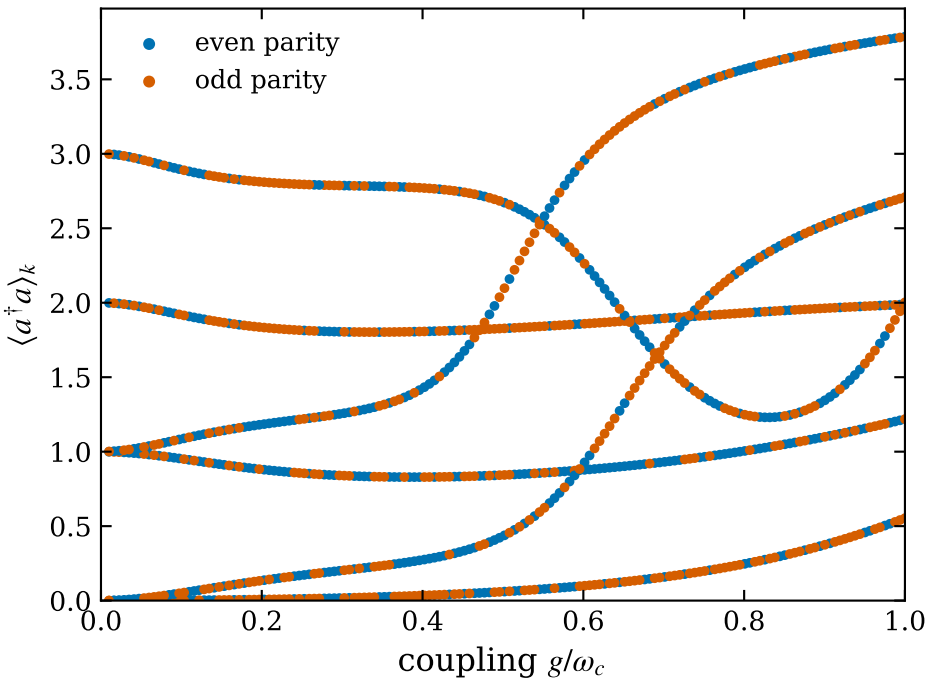
Photon content of the lowest eigenstates, \Delta = 0.7 \omega_c
